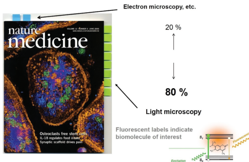
FIGURE 2. Light microscopy remains the most popular microscopy method in the life sciences, due to a number of distinct advantages such as live-cell imaging and biomolecular specificity. The latter is provided by labelling the biomolecules of interest with fluorescent markers, allowing their species-specific detection in the microscope.
