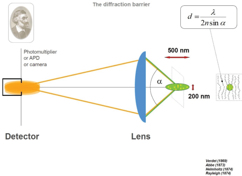
FIGURE 3. Focusing of light by the microscope (objective) lens cannot occur more tightly than Abbe's limit. As a result, all molecules within this diffraction-limited region are illuminated together, emit virtually together, and cannot be told apart.
