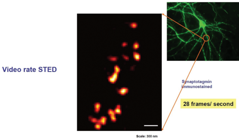
FIGURE 10. Video-rate STED imaging of synaptic vesicle motion in axon of living hippocampal neuron. (Lecture contains video).
