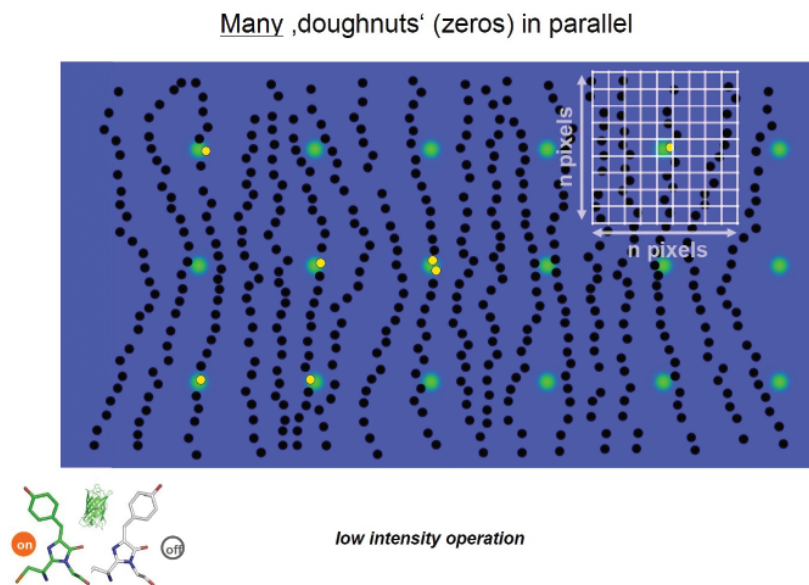
FIGURE 16. Parallelisation of the STED/RESOLFT concept holds the key to faster imaging. The diffraction problem has to be addressed only for molecules residing within a diffraction-limited region. Thus, many intensity minima (‘doughnuts’) are produced, at mutual distances greater than the diffraction limit, for highly efficient scanning of large sample areas. The use of highly parallelised schemes is greatly facilitated by harnessing transitions between long-lived molecular on-off states, such as cis/trans.
