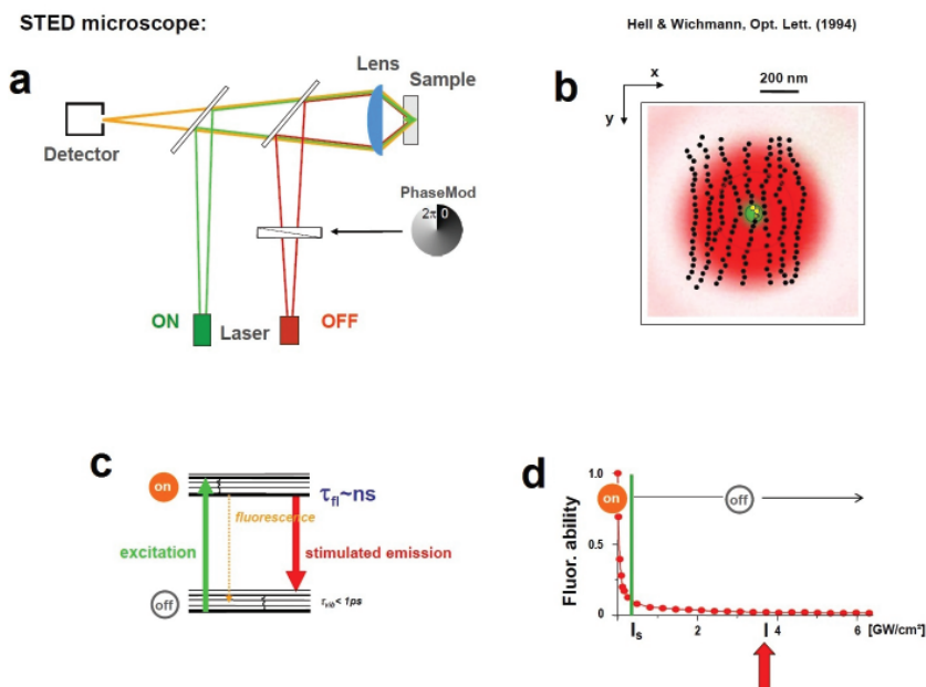
FIGURE 7. STED microscopy. (a) Setup schematic. (b) Region where the molecule can occupy the “on” state (green) and where it has to occupy the “off” state (red). (c) Molecular transitions. (d) For intensities of the STED light (red) equalling or in excess of the threshold intensity I_s , molecules are effectively switched “off.” This is because the STED light will always provide a photon that will stimulate the molecule to instantly assume the ground state, even in the presence of excitation light (green). Thus, the presence of STED light with intensity greater than I_s switches the ability of the molecules to fluoresce off.
