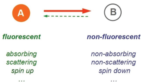
FIGURE 21. The limiting role of diffraction is overcome by utilising at least two molecular states to separate features residing closer than the diffraction barrier. While fluorescent molecules have been the first type of molecules which have provided such states, other molecules and states are conceivable that are not necessarily of the fluorescent type. This is why one could imagine breaking the diffraction barrier also in a non-fluorescence far-field optical microscope, provided suitable states and state transitions are identified.
