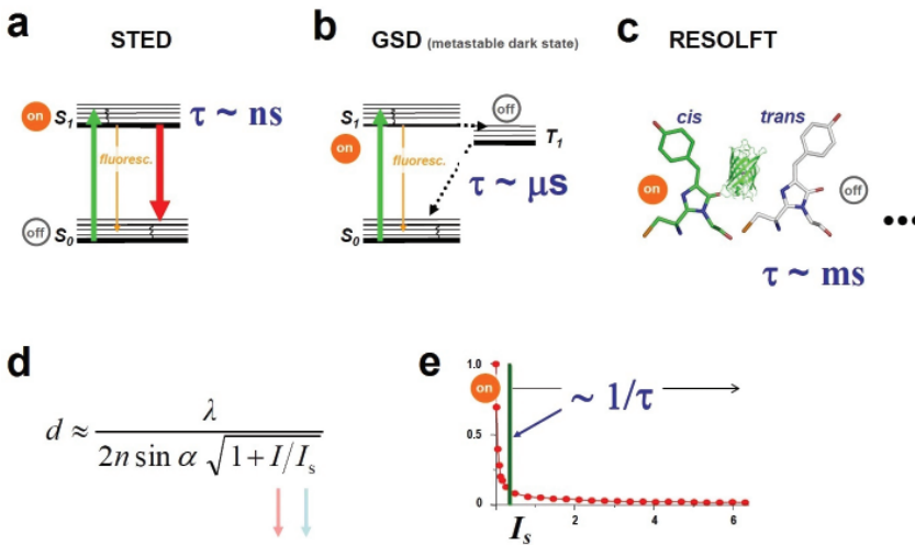
FIGURE 15. States and state transitions utilised in (a) STED, (b) GSD and (c) RESOLFT nanoscopy. (d) The modified expression for the resolution describes the spatial region, in which molecules can still reside in the “on” state. (e) The intensity I_s for guaranteeing the transition is inversely related to the state lifetime. The longer the lifetime of the involved states, the fewer photons per second are needed to establish the on-off state difference which is required to separate features residing within the diffraction barrier.
