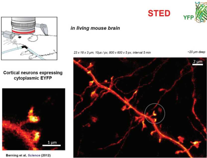
FIGURE 11. STED nanoscopy in living mouse brain.
