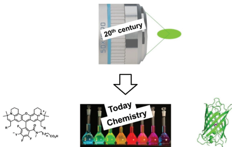
FIGURE 20. From lenses to molecular switches. Whereas in the 20th century, the focusing quality of the lenses was decisive for gaining very high spatial resolution, now it is the molecules and their state transitions which become central to achieving the best resolution. Optimising molecules towards providing robust and repeatedly executable (on/off) state transitions is primarily a chemistry problem.
