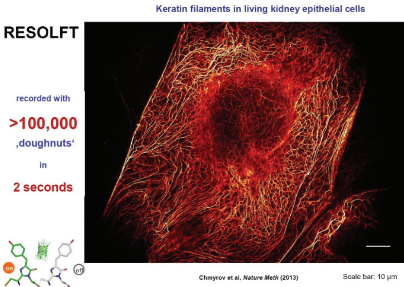
FIGURE 17. Massively parallelised RESOLFT nanoscopy. Here, an array of \sim 114\,000 intensity minima (zeros) was used to image a living cell in two seconds.
