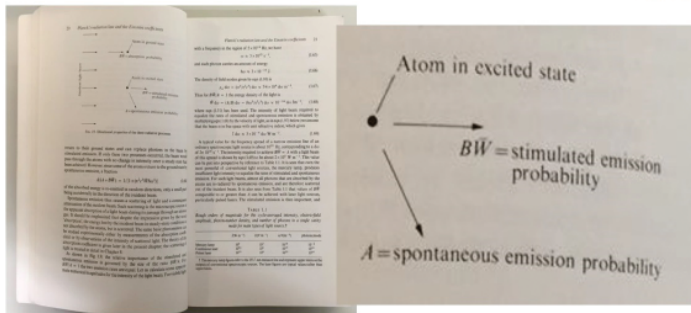
FIGURE 5. Realisation in the early 1990s that the key to surpassing the diffraction resolution limit lies in fluorophore properties (quote from a manuscript submitted in 1993, top). The photograph (bottom) shows page 20 of the book The Quantum Theory of Light by Rodney Loudon (Oxford Science Publications), where I found a reminder of the phenomenon of stimulated emission, which I of course knew about from my physics studies, on Saturday morning, November 6, 1993. My copy of the book is now on display at the Nobel Museum, Stockholm.
