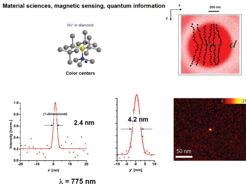
FIGURE 14. Quasi-ideal fluorophores, in particular virtually unlimited repetitions of the resolution-enabling on-off state transitions, provide the present resolution records in far-field optical imaging using STED, in the single-digit nanometre regime. Color centres (charged nitrogen vacancy centres) in diamonds hold great potential for various other applications, notably in magnetic sensing and quantum information, which may be combined with diffraction-unlimited lens-based (far-field) optical readout.
