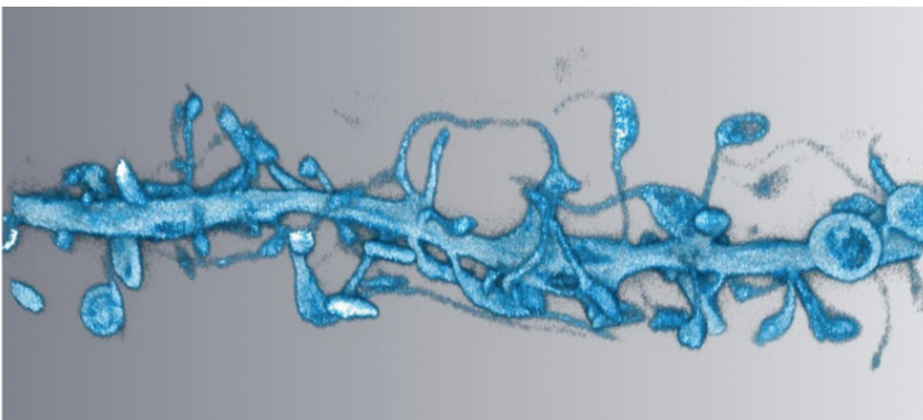
FIGURE 12. Rendition of three-dimensional STED nanoscopy data showing the dendritic actin from a neuron of a living organotypical hippocampal brain slice (mouse).
