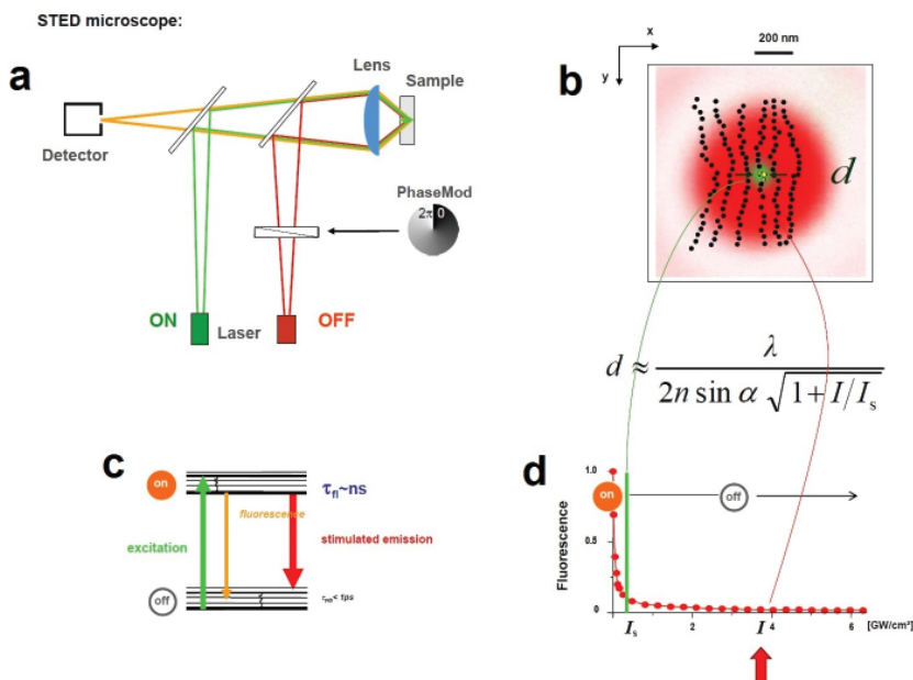
FIGURE 13. Resolution scaling in the STED/RESOLFT concepts: an extension of Abbe's equation. The resolution scales inversely with the square-root of the ratio between the maximum intensity at the doughnut crest and the fluorophore-characteristic threshold intensity I_s .
