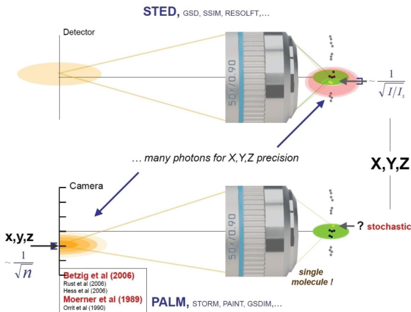
FIGURE 19. Both in coordinate-targeted and in coordinate-stochastic nanoscopy methods, many photons are required to define or establish molecular coordinates at subdiffraction scales. In the coordinate-targeted mode (STED, RESOLFT, etc.), the coordinates of (e.g.) the “on”-state are established by illuminating the sample with a pattern of light featuring an intensity zero; the location of the zero defines the coordinates with subdiffraction precision. In the coordinate-stochastic mode (PALM, STORM etc.), the coordinates of the randomly emerging “on”-state molecules are established by analysing the light pattern emitted by the molecules (localisation). Precision of the spatial coordinate is achieved in both cases by a sufficient number of photons. In both families, neighbouring molecules are discerned by transiently creating different molecular states in the sample.
