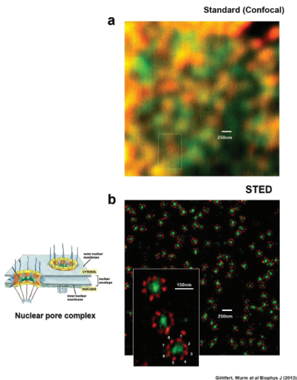
FIGURE 8. Nuclear pore complex architecture in an intact cell nucleus imaged by (a) confocal microscopy (diffraction-limited), and (b) STED nanoscopy.
