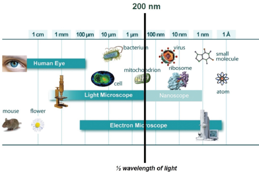
FIGURE 1. Length scales and spatial resolution limits of visual inspection (human eye), light (optical) microscopy and electron microscopy. Far-field optical nanoscopy extends the resolution much beyond Abbe’s limit of half the wavelength of light used (~200 nanometres).
