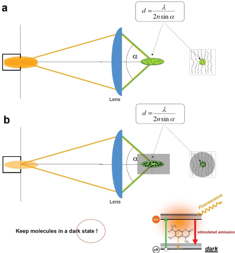
FIGURE 6. Switching molecules within the diffraction-limited region “off” enables the separate detection of neighbouring molecules residing within the same diffraction region. (a) In fluorescence microscopy operating with conventional lenses (e.g. confocal microscopy), all molecules within the region covered by the main diffraction maximum of the excitation light are flooded with excitation light simultaneously and emit fluorescence together. This is because they are simultaneously allowed to assume the fluorescent (signalling) state. (b) Keeping most molecules—except the one(s) one aims to register—in a dark state solves the problem. The dark state is a state from which no signal is produced at the detector. Such a transition to the dark “off” state is most simply realised by inducing stimulated emission, which instantaneously forces molecules to their dark (“off”) ground state.
