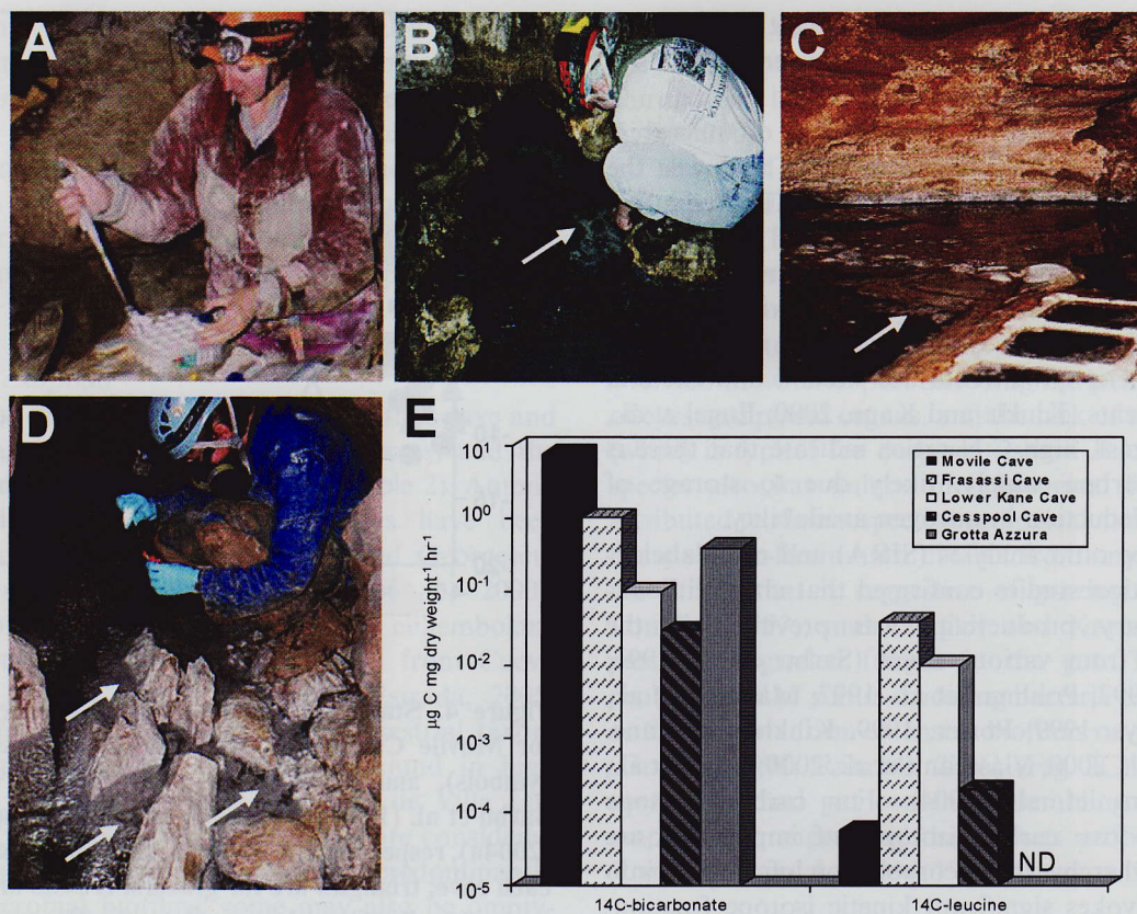
Figure 5. (A) Set-up for radiolabelled-isotope experiment in the Frasassi Caves, Italy. (B) Sampling in Cesspool Cave, Virginia; arrow pointing to mats. (C) Floating microbial mats (arrow) in Movile Cave, Romania. Grid is ~10 cm on a side. (D) Sampling stream mats in the Frasassi Caves, Italy; arrows pointing to mats. (E) Comparison between cave microbial mats for 14 C-bicarbonate and 14 C-leucine incubations to estimate chemolithoautotrophic primary productivity and heterotrophic productivity, respectively (Porter, 1999). Autotrophic productivity only was estimated for Grotta Azzura, Italy (ND = no data for leucine test) (Mattison et al., 1998).
